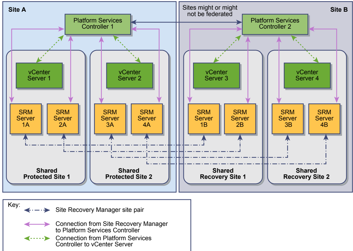
Figure 10-3. Site Recovery Manager in a Shared Protected Site and Shared Recovery Site Configuration
