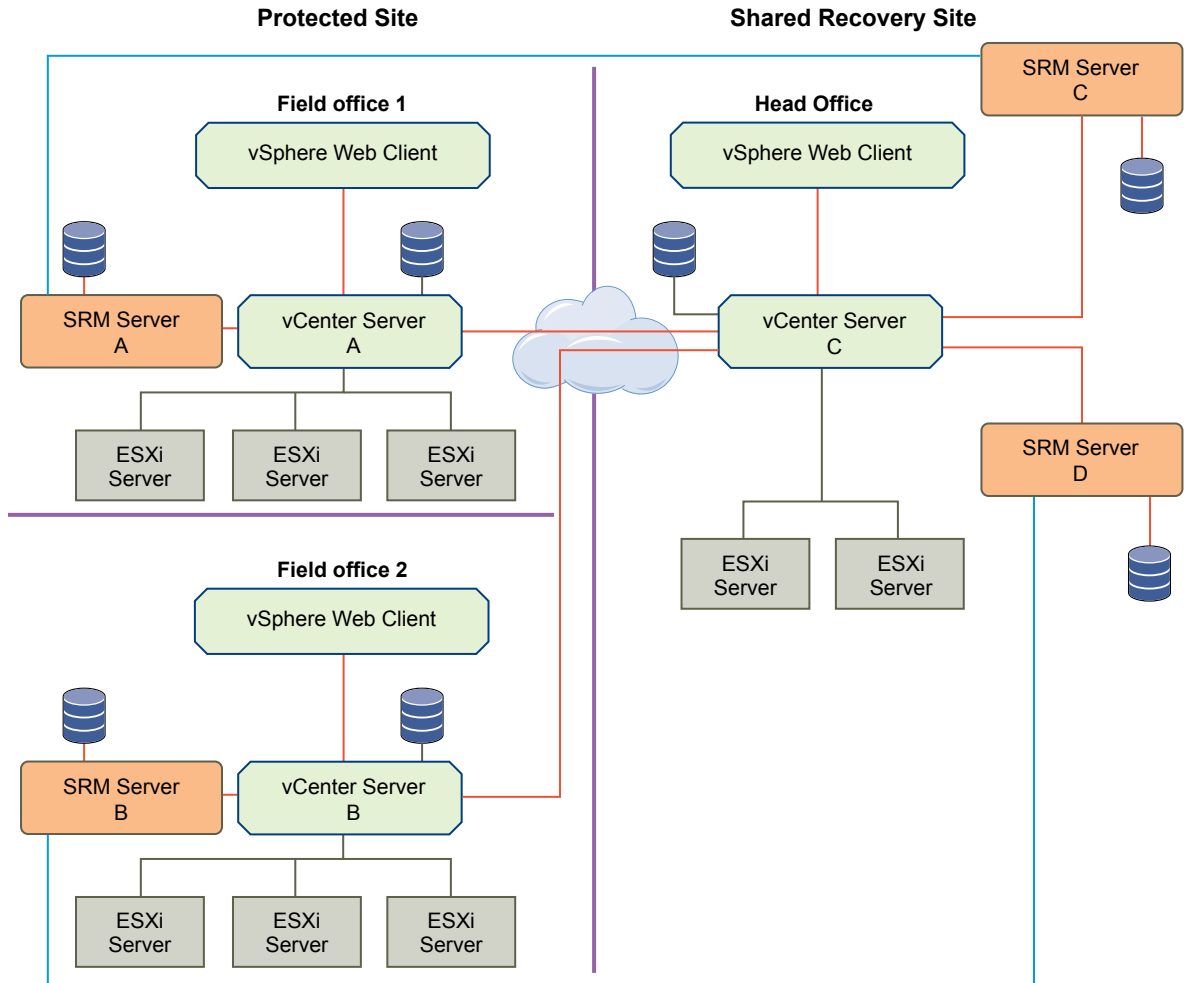
Figure 10-1. Example of Using Site Recovery Manager in a Shared Recovery Site Configuration
