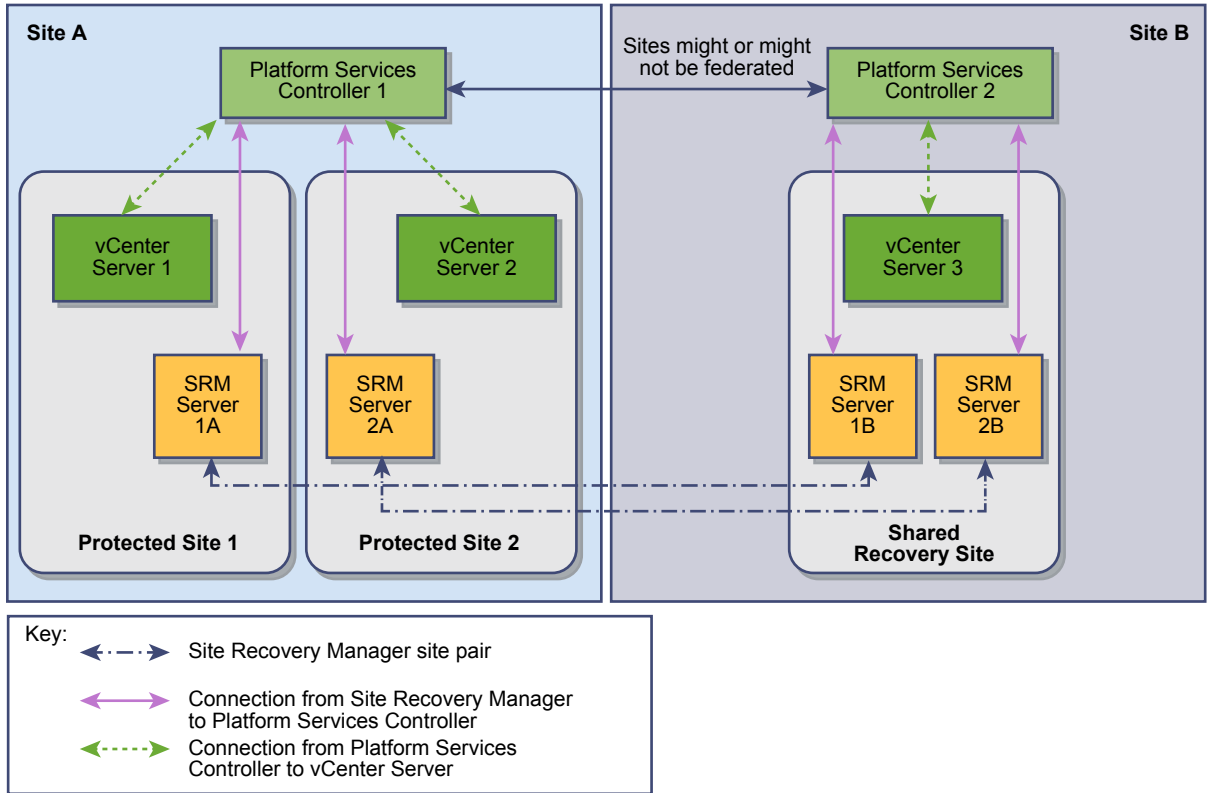
Figure 10-2. Site Recovery Manager in a Shared Recovery Site Configuration
