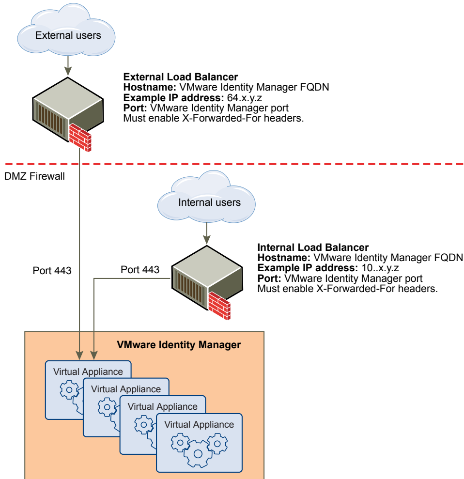
Figure 7-1. External Load Balancer Proxy with Virtual Machine
